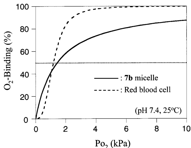
Fig. 3. The O_2 -binding equilibrium curves of the 7b micelle and red blood cells.
