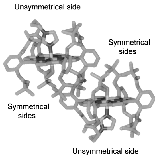
Fig. 2. Proposed structure of the 7b micelle center which consists of the dimeric porphyrin moieties. The laterally slipped stacking geometry of the symmetrical side (Fe–Fe distance: 1.3 nm) is based on the results in Ref. 1b.
