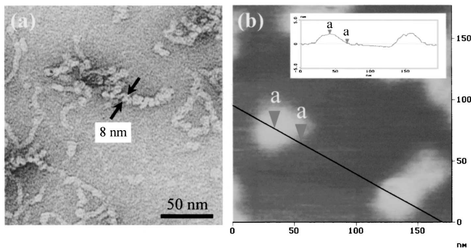
Fig. 1. (a) TEM of the evaporated 7b micelle stained by uranyl acetate, and (b) SFM image (tapping mode) of the evaporated sample of the 7b micelle on HOPG surface. Image size is 180 \times 180 \text{ nm}^2 and vertical a-a distance is 1.96 nm.
